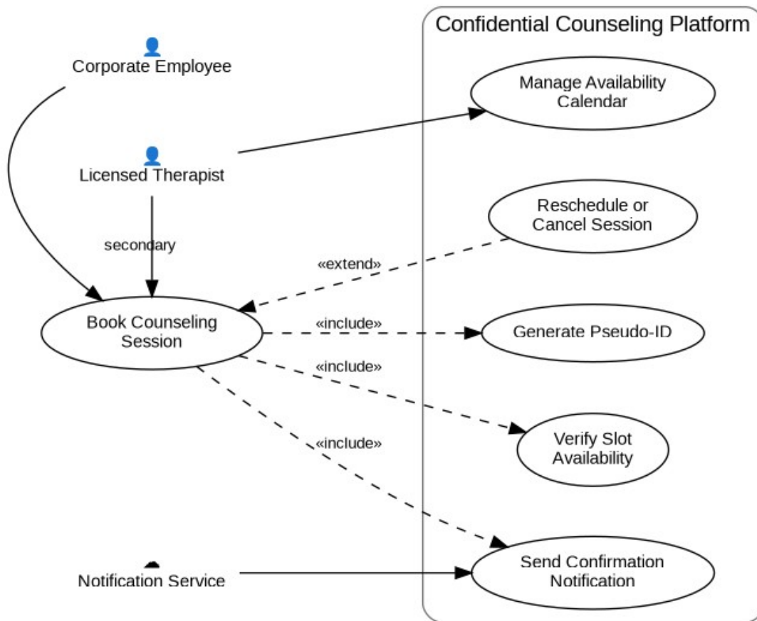
Figure 1. UML Use-Case Diagram
