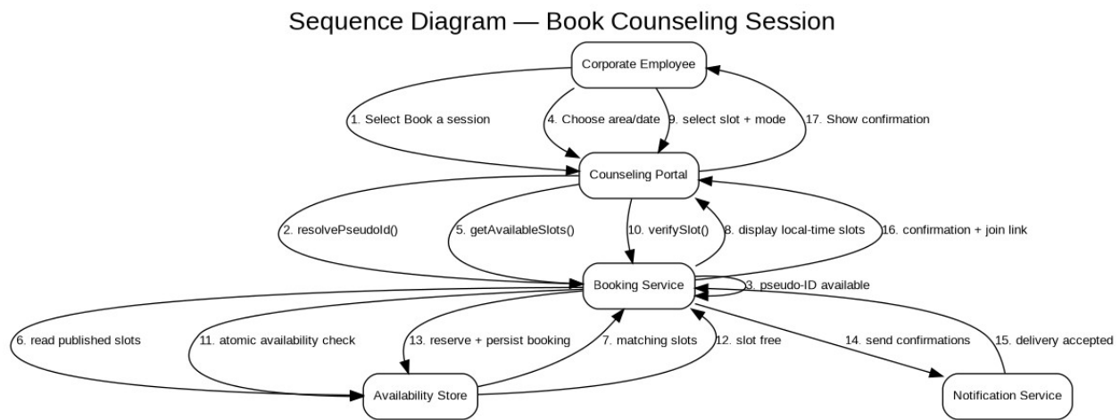
Figure 3. Sequence Diagram for UC-03
